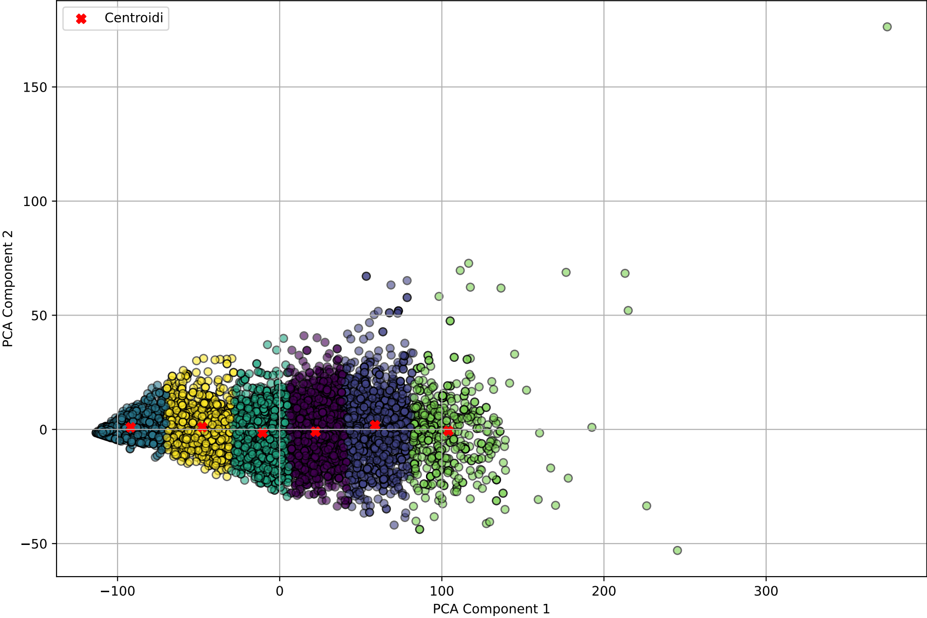
K-means Clusters in PCA Projection (all wines)
